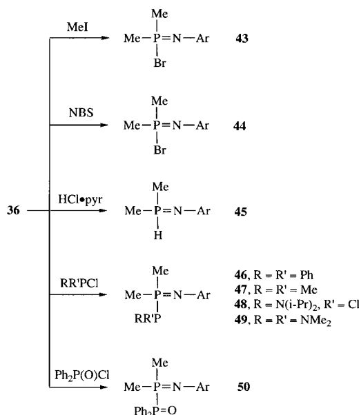
Scheme 12.
